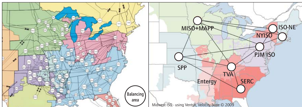
Figure 21 • Balancing areas in the eastern United States in 2007 (left), and assumed in 2024 (right)
