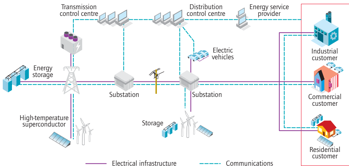
Figure 19 • Power system interaction through an intelligent grid
