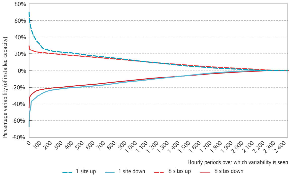
Figure 28 • Impact of geographical spread smoothing PV variability
