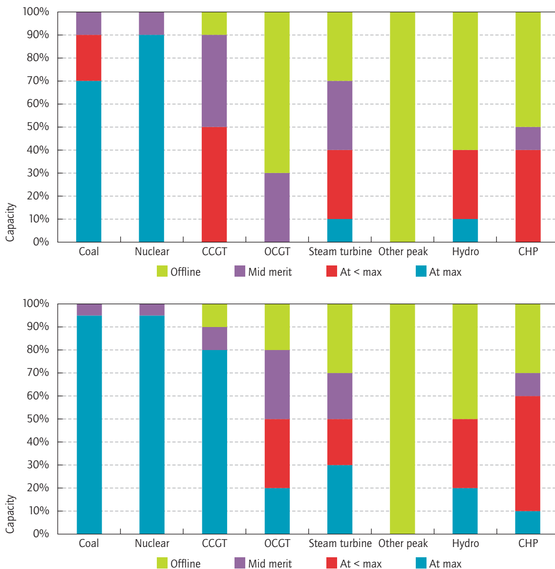
Figure 55 • Likely operation of dispatchable plant (Mexico) at minimum demand (top figure), and peak (bottom figure)
