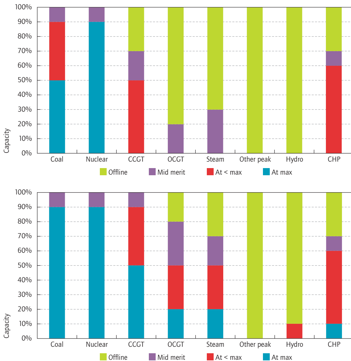
Figure 39 • Likely operation of dispatchable plant (British Isles) at minimum demand (top figure), and peak (bottom figure).
