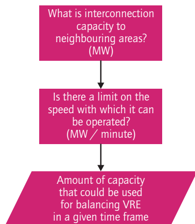
Figure 10 • Flexible resource in interconnections
